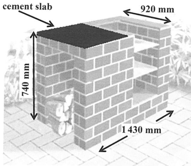
Picture of braai stand
