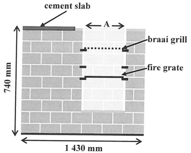
Front view of braai stand
